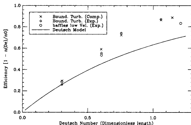
Figure 15. Wire-plate precipitator.
