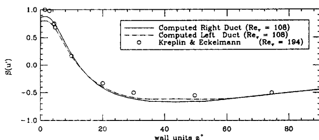
Figure 6. Skewness of the streamwise fluctuating velocity.
