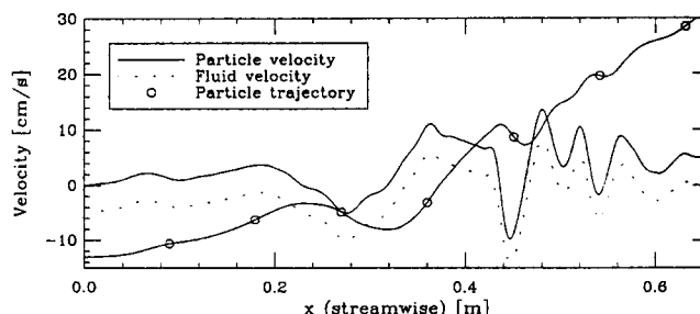
Figure 8. Plate-plate precipitator.
