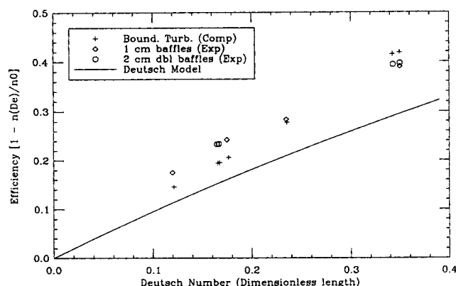
Figure 11. Plate-plate precipitator.
