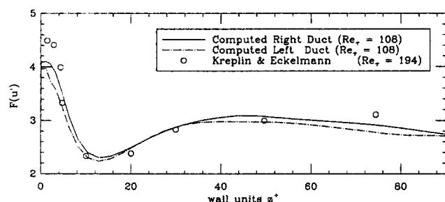
Figure 7. Flatness of the streamwise fluctuating velocity.
