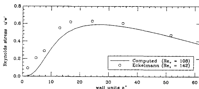
Figure 4. Reynolds stress ( u'w' ).
