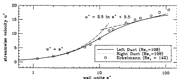
Figure 3. Mean streamwise velocity.
