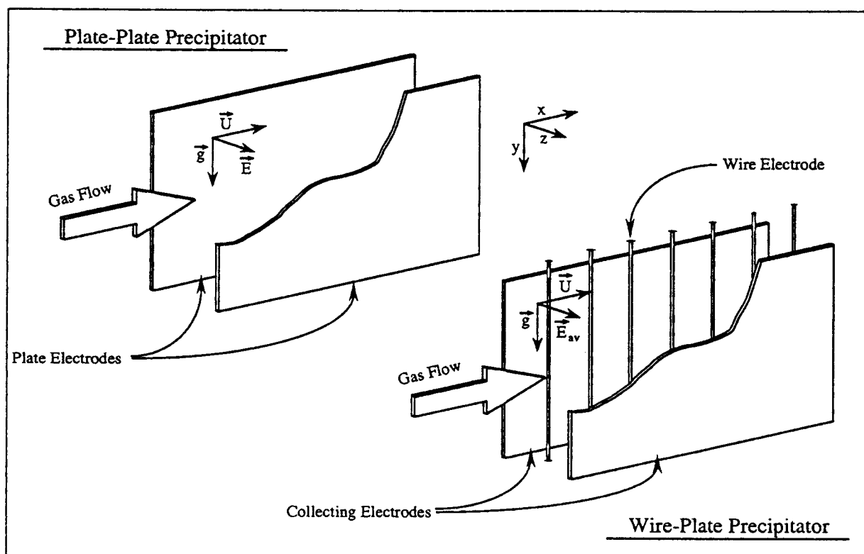
Figure 2. Plate-plate and wire-plate precipitator geometries.
