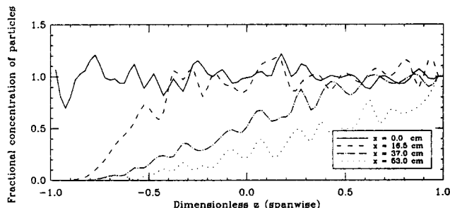
Figure 9. Plate-plate precipitator.
